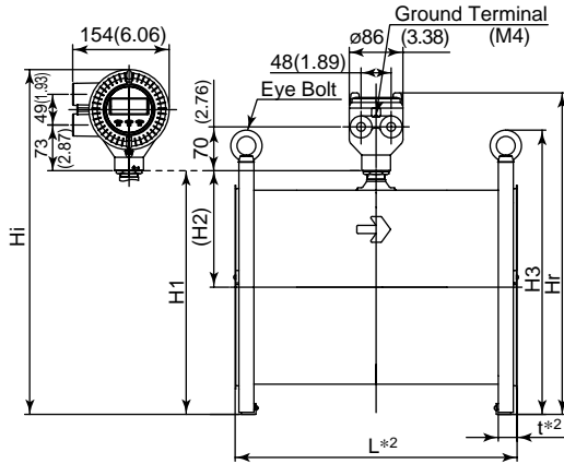
Integral Flowmeter Remote Flowtube
