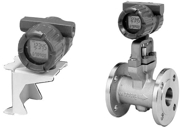
Model DYA Remote Type Converter
