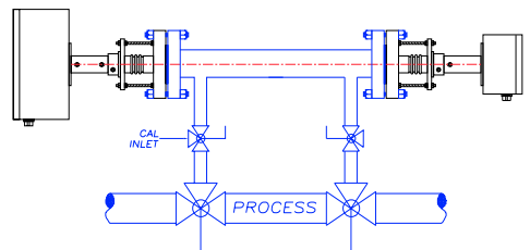
Bypass/Close Coupled Extractive
