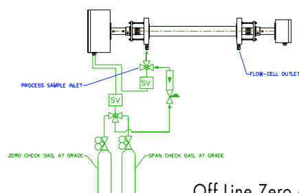
Off Line Zero and Span (Controlled and Recorded by Analyzer)
