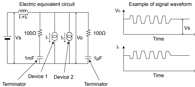
Figure 2.5 Electric Equivalent Circuit of Signal Transmission
