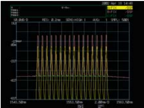
WDM waveform before/after amplification by EDFA
