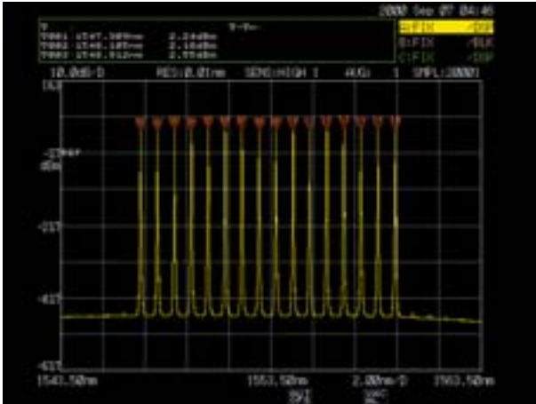
WDM measured waveform
