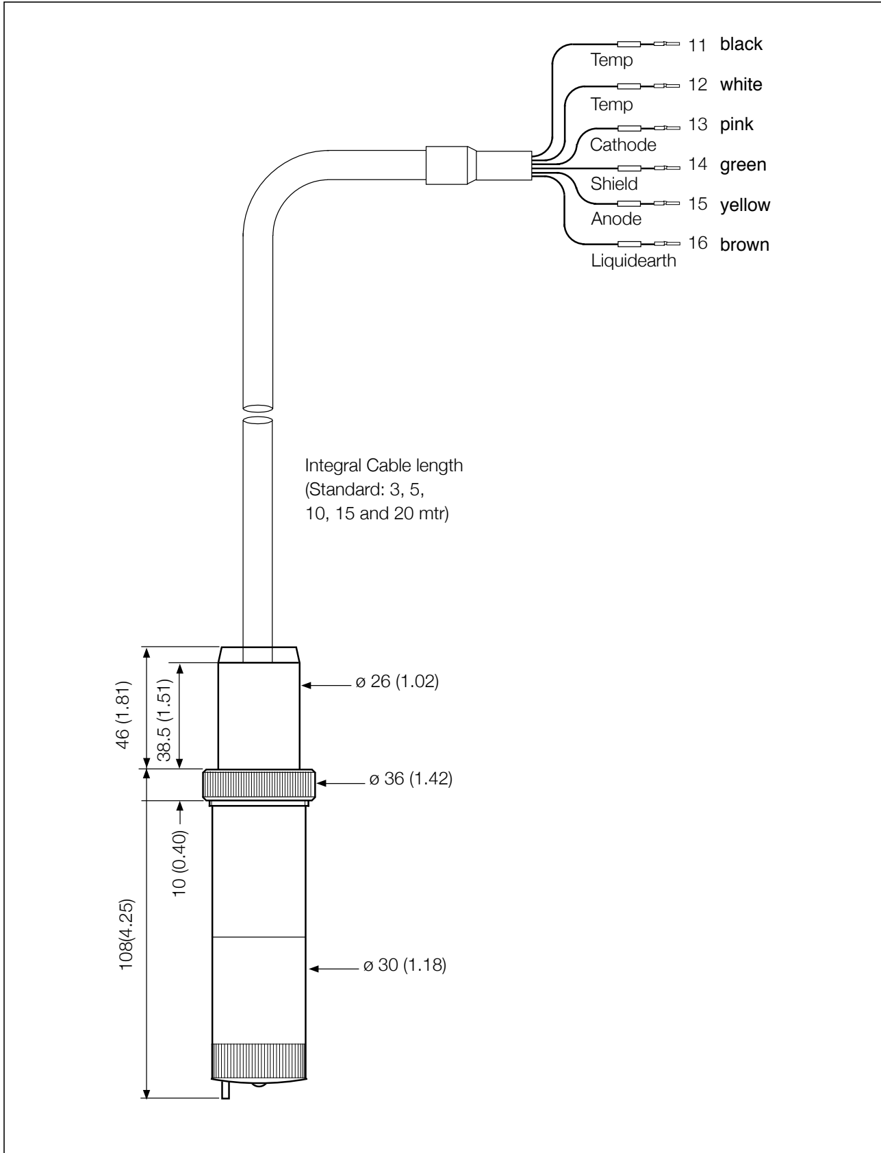
Figure 1. DO30G sensor
