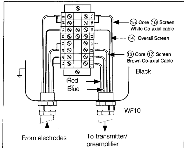
Connection diagram
