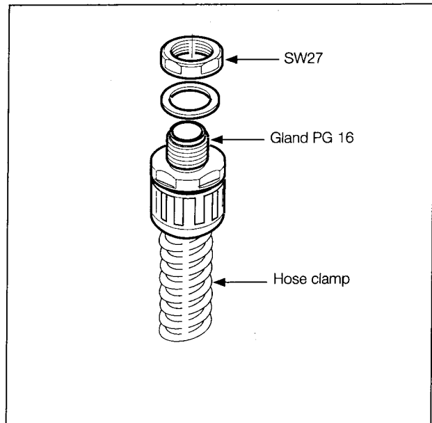
Hose connection
