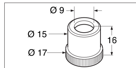
Fig.12. K1500DW (set of 12 cable nuts).
