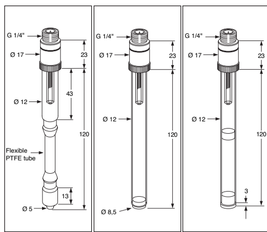
Fig.1 SR20-AC22 Fig.2. SR20-AP24 Fig.3 SR20-AP26
