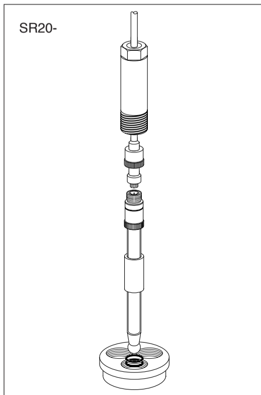
Figure 8. Standard mounting options
