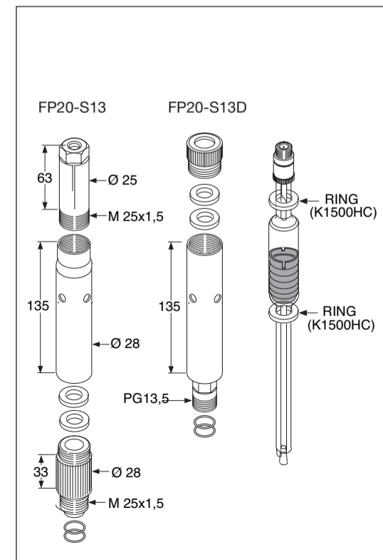
Figure 11. Mounting kit SR20-AC32
