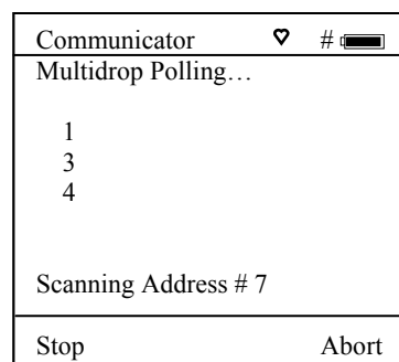
Multidrop Polling Screen Multidrop & Burst Mode Support
