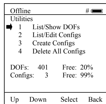
HART Offline Menu Screen
