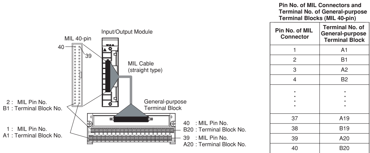
Figure Correspondence between the Signal Lines of MIL (40-pin) Connectors and Those of General-purpose Terminal Blocks
