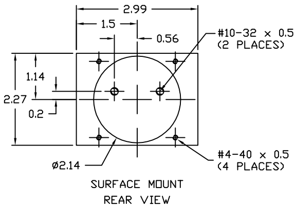
FIG. 9-A STYLIST SERIES TYPES 260,261,264, & 265. (2 1/2)
