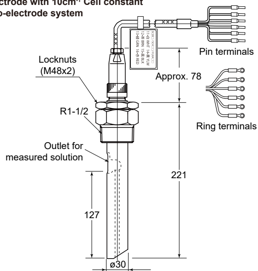
Unit: mm
