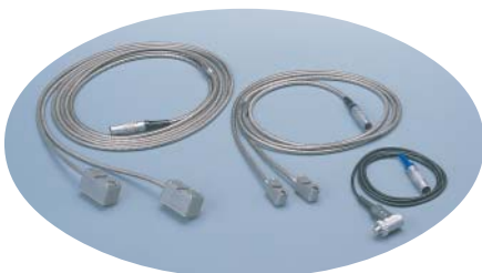
Left: Transducers for large pipe Middle: Transducers for small and medium pipe Right: Wall thickness probe (for general temperature)
